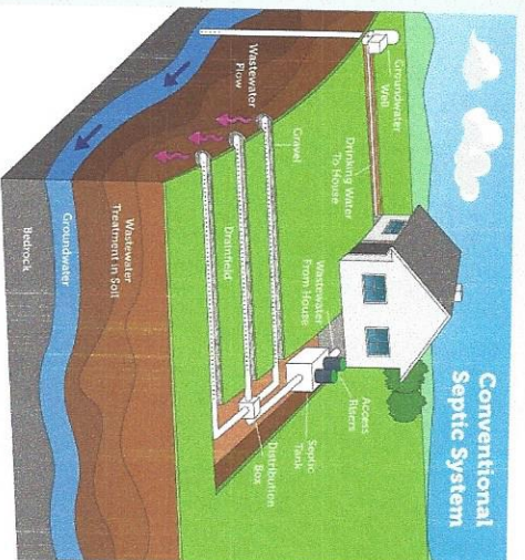
Septic graphic from epa.gov
